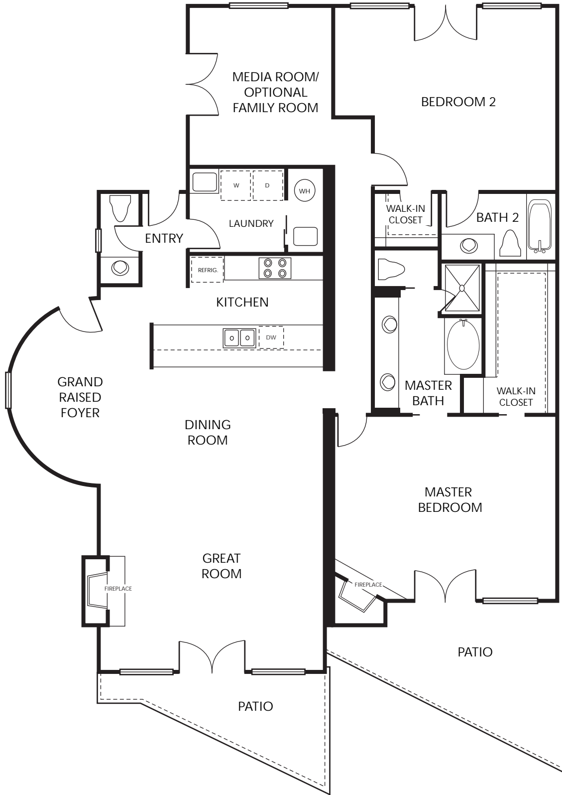
1 Story Plan
